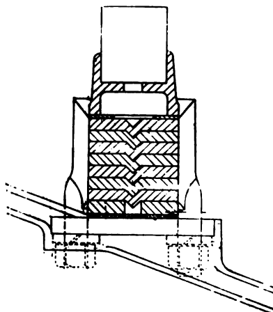
Section of Springs.
